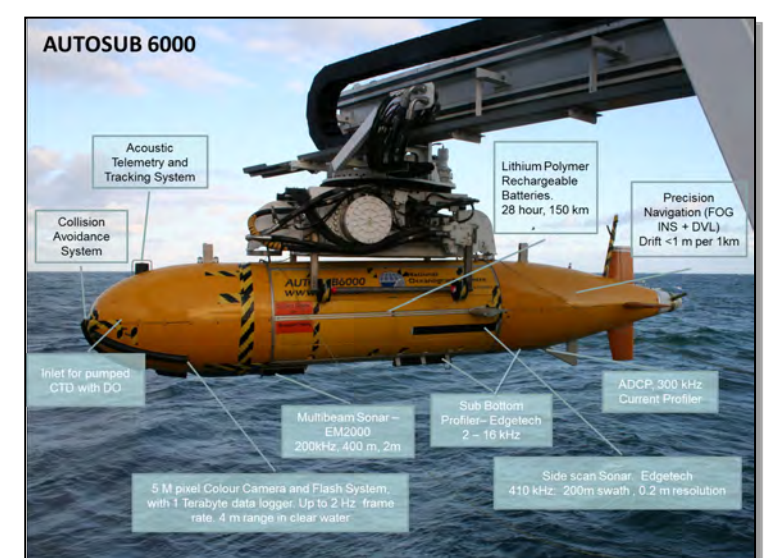
The AUV Autosub 6000 equipped with sensors for detecting shallow fluid flow (image courtesy NOC Southampton).
